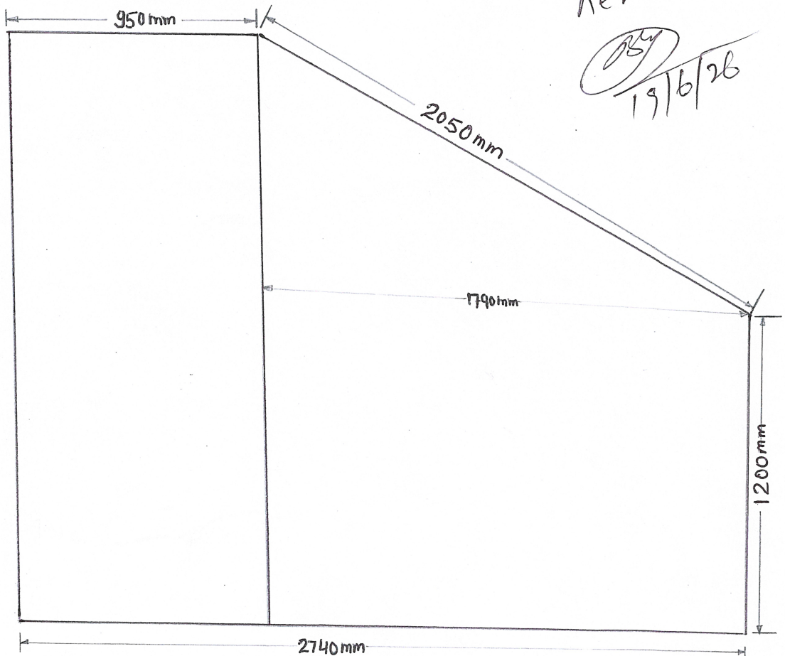
SIDE ELEVATION
